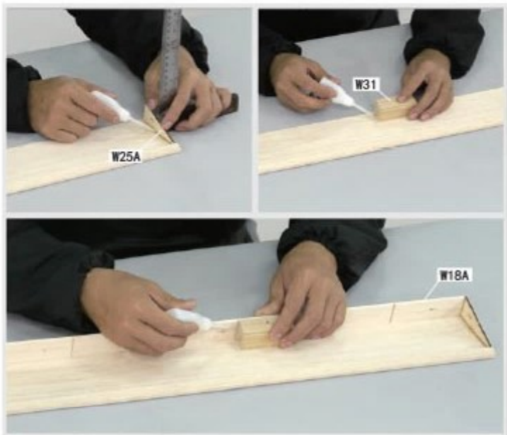
1.29 Glue W25A in place at both ends. Glue W31 to W35A opening, then glue W18A in place. Make sure W31 tapers towards the trailing edge.
