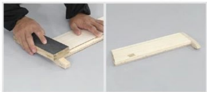
3.16 Remove rough edges with sand paper.
