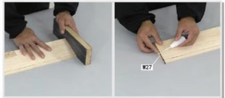
1.32 Remove rough edges at both ends with sand paper, the glue W27 in place.
