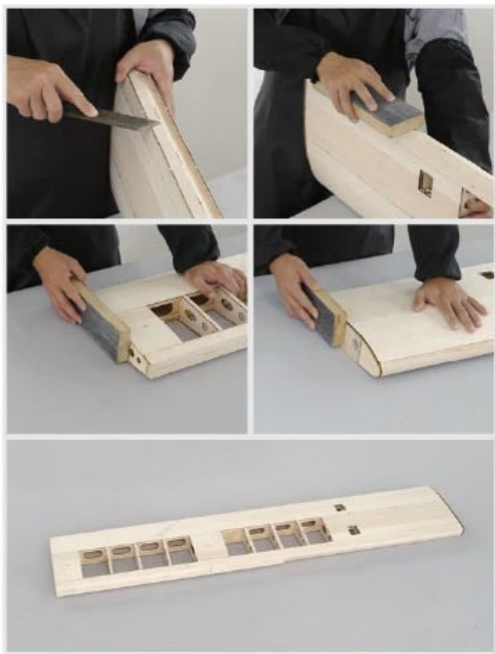
1.18 When glue is cured, cut and remove rough edges with sand paper.
