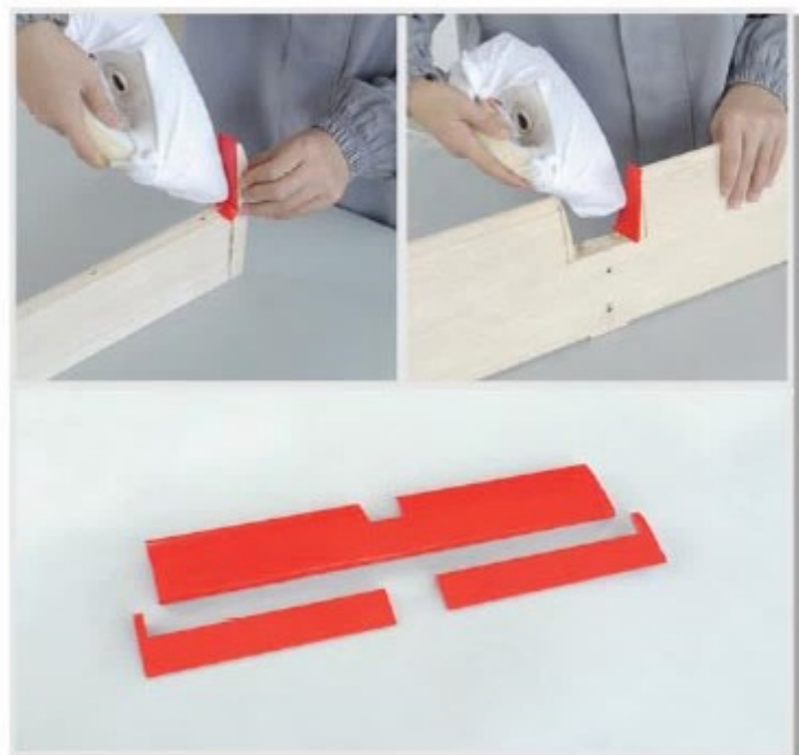
6.16 Cover horizontal stabilizer and elevator.
