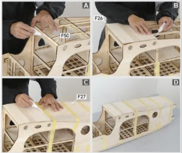
4.26 Glue in F5C, when cured glue in F26. Apply slow curing glue to surfaces in contact with F27. Apply moisture to outer 6 cm portion of F27 then put on top of frame. Use tape to keep F27 in position, more tape on curved section. When cured apply glue for reinforcement.
