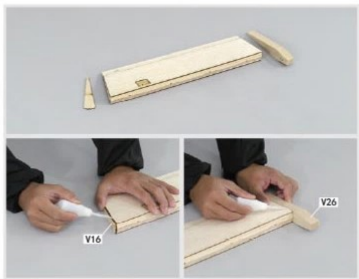
3.15 When cured, glue in V16 an dV26.
