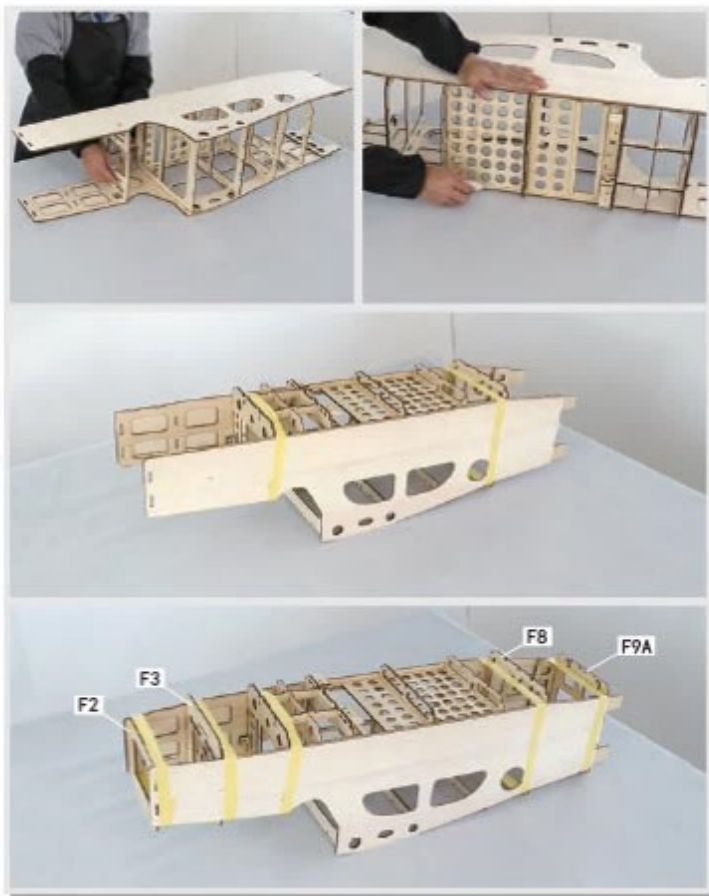
4.17 Insert right side frame into left side panel. Make sure all latches are inside corresponding slots and apply glue. Use tape to secure the side panel. Glue in F3, F2, F8 and F9A. Use tape to force side panels to curve in to conform with F3, F2, F8 and F9A.
