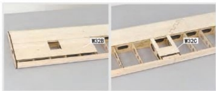
1.15 Glue W32B and W32C in place. Flip over wing and add glue to all surfaces in contact.
