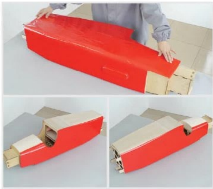
6.5 Use similar procedure to cover the left and right side of fuselage. Note that the total overlap of coverings at seams will be 6 mm.
