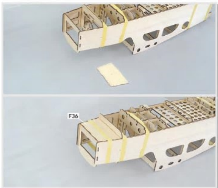
4.19 Flip over fuselage and glue in F36.
