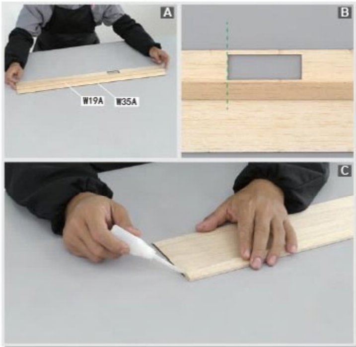
1.28 Align W19A slots with W35A opening. Glue W19A to W35A.
