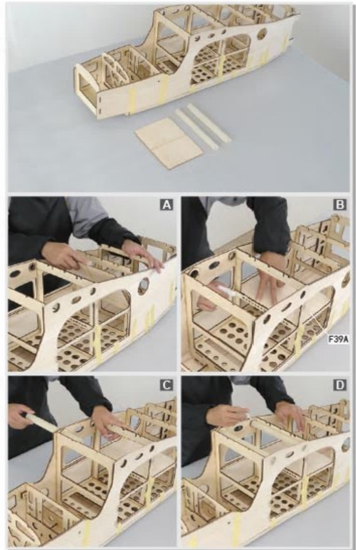
4.24 Glue in F39A and wing tube sleeve.
