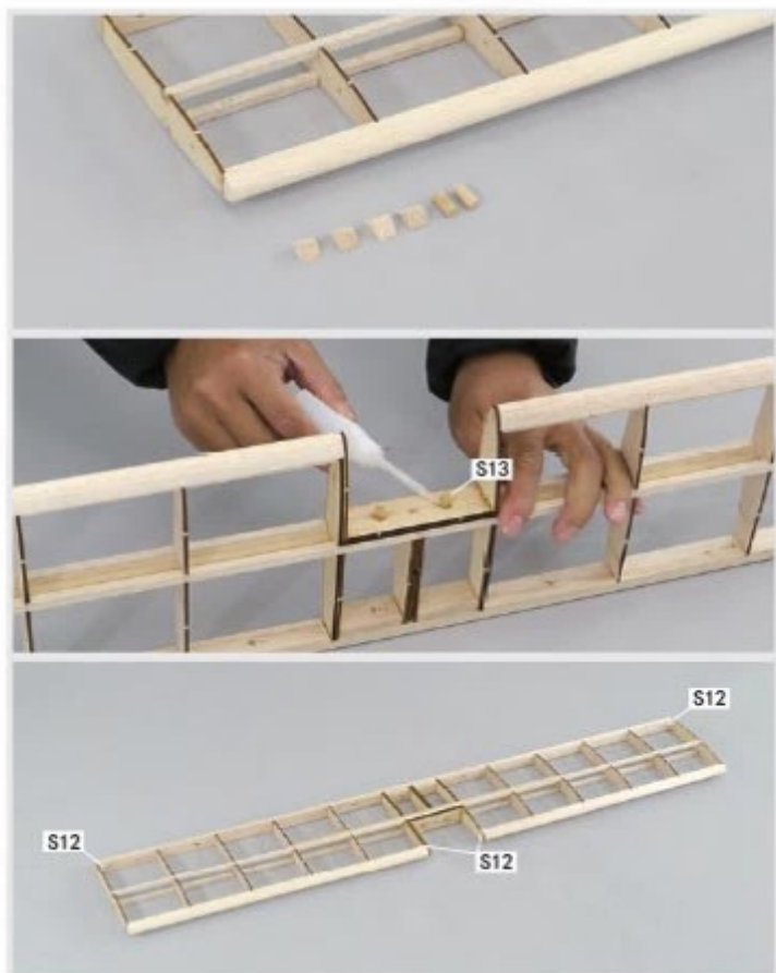
2.6 Insert S13 into round holes and apply glue. Glue S12 in place.
