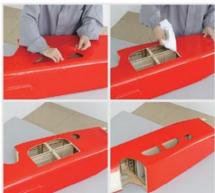
6.7 Cut openings for windows. Allow 3 mm overlap and iron on rim of windows.
