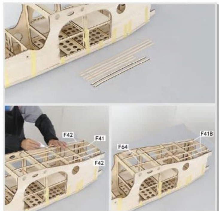
4.25 Glue in F41, F41B, F42 and F64.
