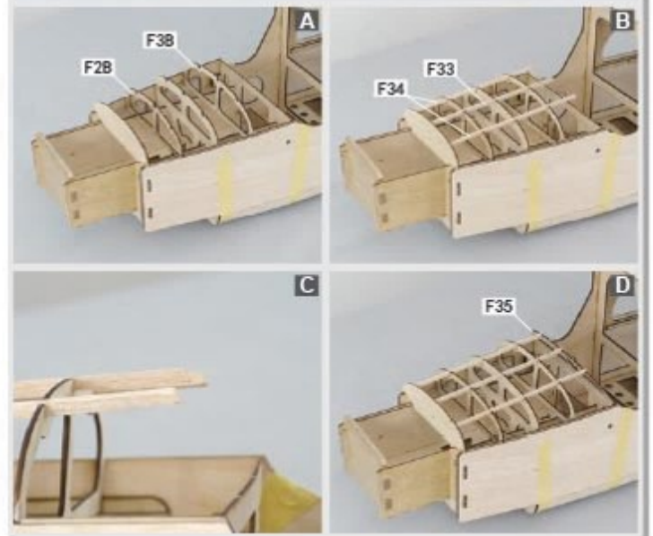
4.28 Glue in F2B and F3B. Glue in F33 and F34. Make sure tapered surface is facing outwards. Then glue in F35.
