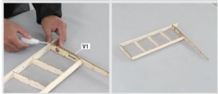
3.2 Glue V1 and V6 in place. Make sure plywood side of V1 is facing V2.
