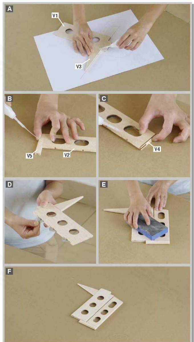
Lay out parts for the vertical fin and rudder
