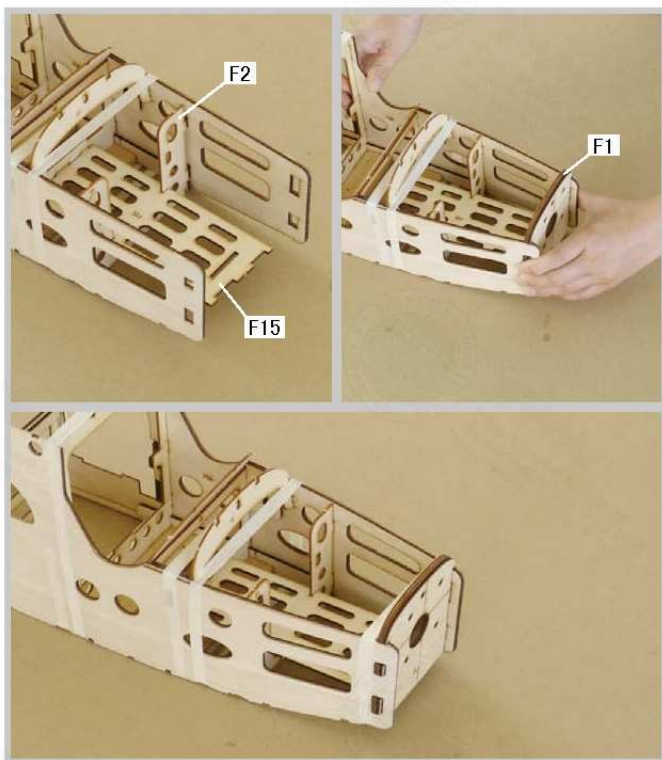
1.19 Latch in F2, F15 and F1 into side panels and hold them in position with tape. Make sure the blind nuts at F1 is facing the rear. For better strength of the firewall, it is recommended to use epoxy to glue F1 to the side panels.
