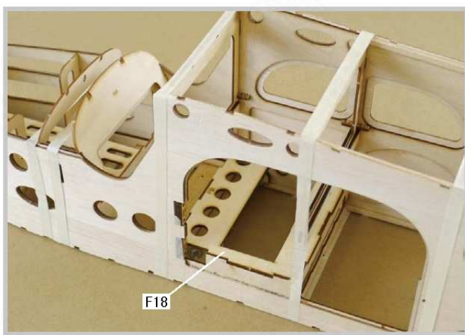
1.21 Glue in F18.
