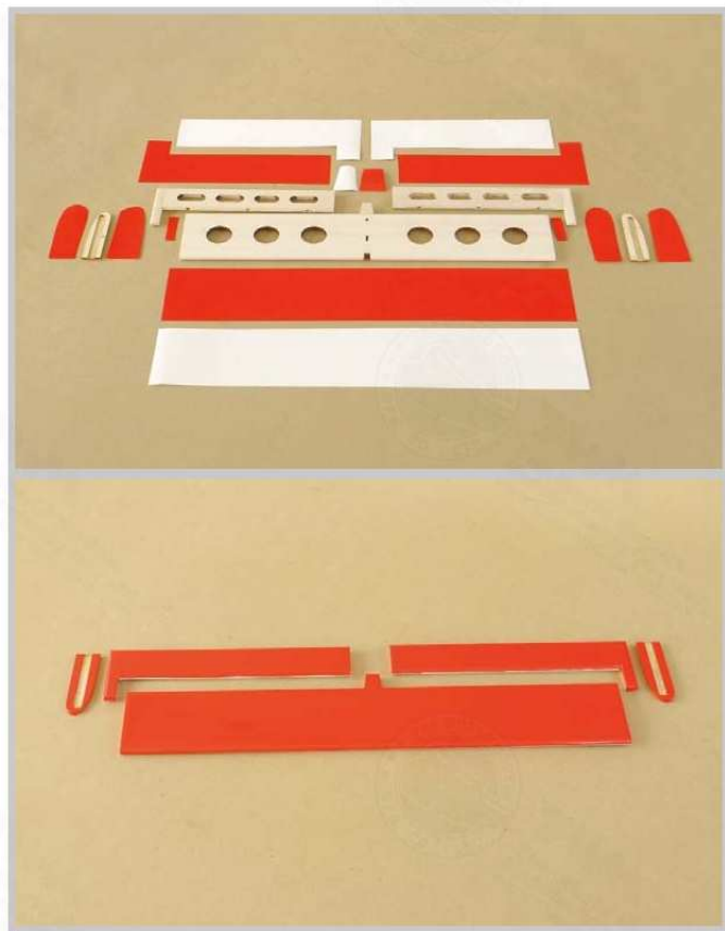
11.16 Cover the horizontal stabilizer and elevator.
