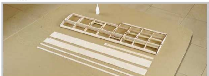
6.6 Flip over right wing with wing bottom up. Latch in W19 to W5R, with blind nut facing inside wing. Apply CA to glue in place. Glue in W16. When cured flip over wing to bottom down, glue in 4x F18 and add CA to all contact surfaces.
