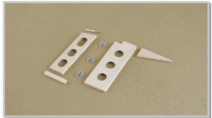
Lay out parts for the vertical fin and rudder
