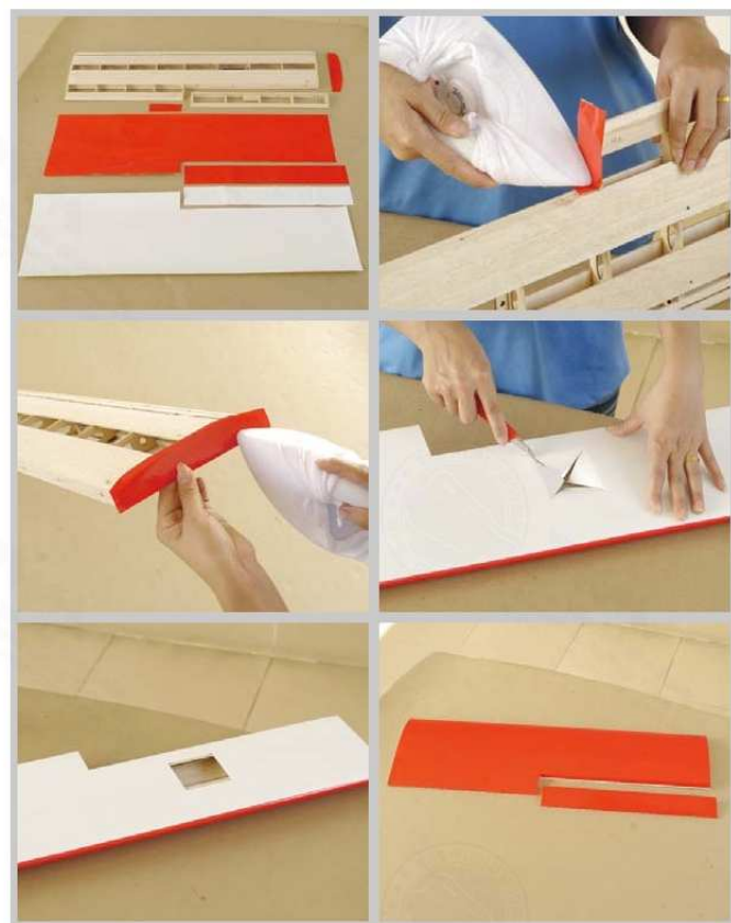
11.12 Cover the right wing panel. Cover the wing tip first, then the bottom panel, and then the top panel. Cover the ailerons the same way, tip first, then bottom and then the top. Cut opening for the aileron servo tray. Leave overhangs and iron on to cover the rims.
