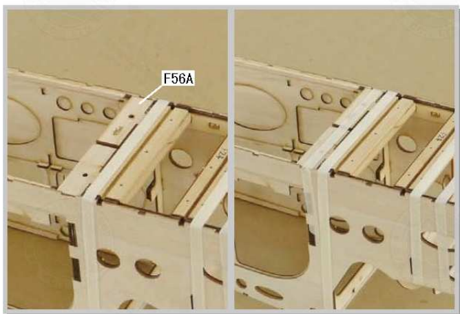
1.16 Flip fuselage over and latch in F56A, note that the blind nuts should be facing inward of the fuselage.
