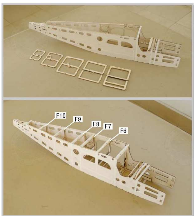
1.17 Latch in F6, F7, F8, F9 and F10 between the fuselage panels. Pay attention to the tenons and cut outs, they may not be symmetrical and if they don't seem to fit, flip it left to right will do.
