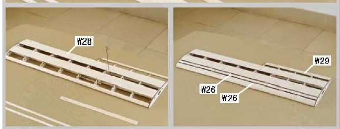
6.7 Glue in W27 and W28, use straight rule to make sure surface is straight. Align the pre-drill holes on W27 and W28 with holes on W4R, they are for the wing bolts. Glue in W26 and W29.
