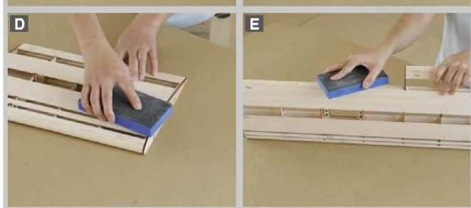
6.9 Glue in W1B. Insert the two wing tube to align the wing tube holes. Use CA to fix W1B in position, remove the wing tubes and apply more CA to glue it in place. Use sand paper to remove rough edges.
