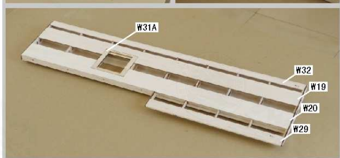
6.8 Flip over wing with bottom up, glue in W31A, W32, W19, W20, W29. Align the hole on W19 with the blind nut hole for wing strut installation. Apply CA to glue all surfaces in contact.
